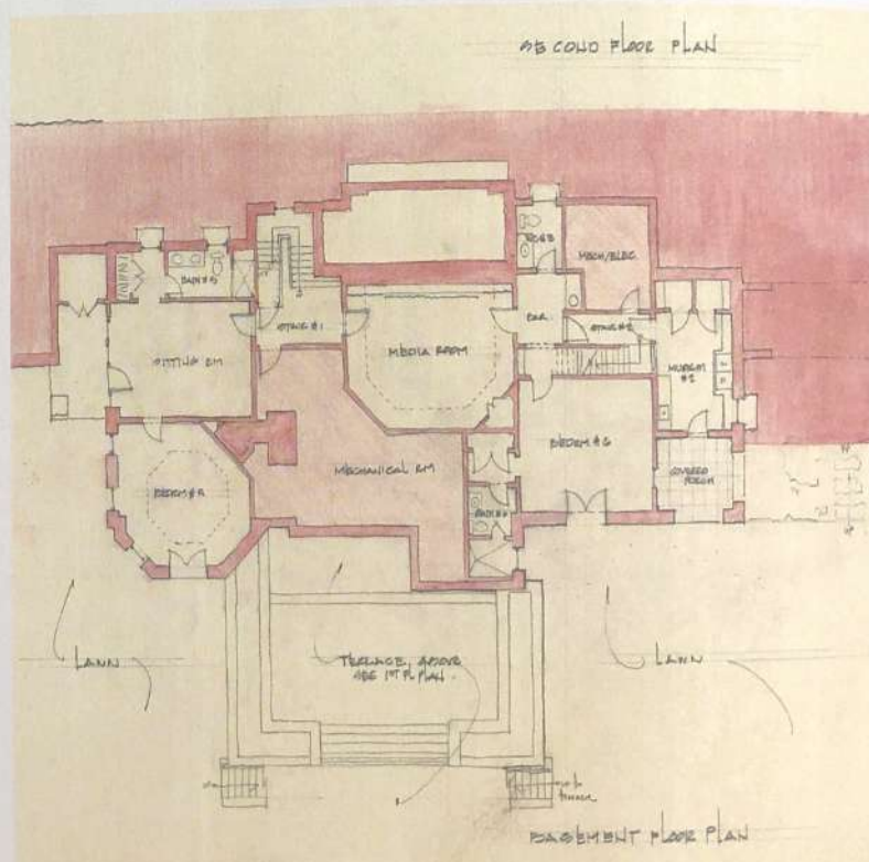
Architectural floor plan
